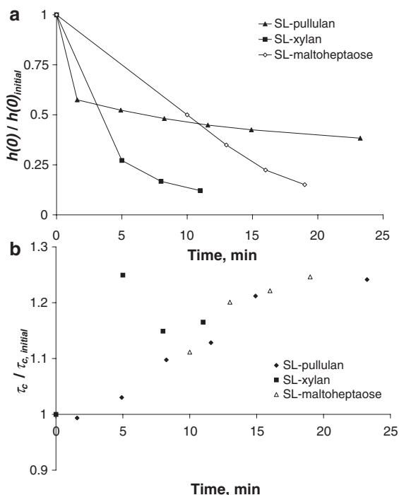
Fig. 7. (a) Relative change in h(0) of SL-polysaccharides in the presence of muddy sediments. h(0) of the polysaccharide in seawater was taken as the reference value h(0)_{\text{initial}} . (b) Relative changes in rotational correlation times of SL-polysaccharides in the presence of muddy sediments. Rotational correlation times of the polysaccharide in seawater were taken as the reference value.
