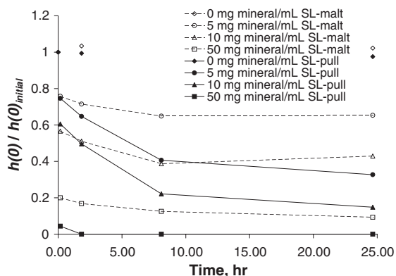
Fig. 8. Relative changes in the h(0) of SL-pullulan and SL-maltoheptaose dissolved in ASW in the presence of montmorillonite, as a function of time. h(0) of the appropriate polysaccharide immediately after it was dissolved in ASW was used as the reference value. In order to facilitate comparison of EPR spectra, the concentration and quantity of SL-polysaccharide solution was kept constant, while the quantity of montmorillonite was varied. Unbroken lines and filled symbols indicate SL-pullulan; dashed lines and open symbols indicate SL-maltoheptaose. Diamonds: zero montmorillonite present, circles: 5 mg montmorillonite/mL polysaccharide solution, triangles: 10 mg mL, squares: 50 mg mL -1 .
